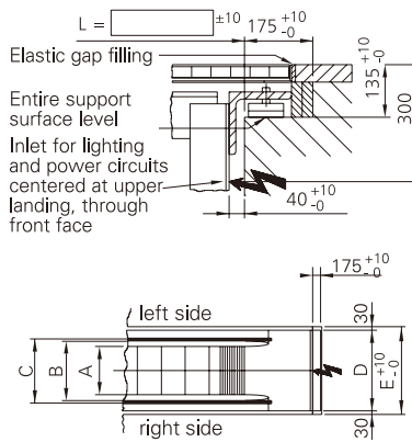
Detail Z
